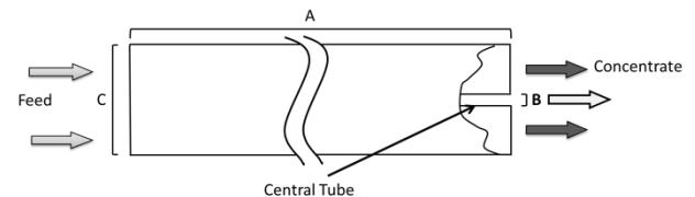
Figure 2: Element Dimensions Diagram – All Except 8040
