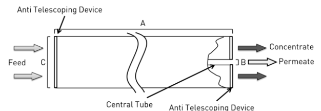
Figure 1: Element Dimensions Diagram – 8040
